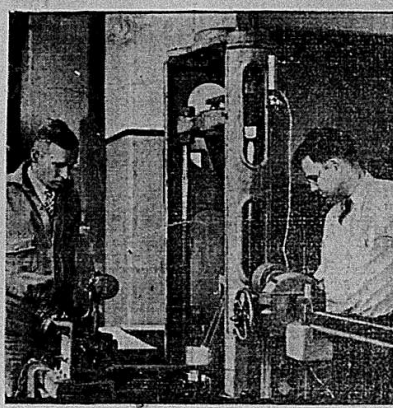
Pintles which support the massive gates of locks in the interior waterways are being tested by the bureau of standards in an effort to discover new combinations of metals which will give the best service. Dr. A. H. Strang, in the leather jacket, is assisted by L. R. Sweetman as tests are made for gates on the Pickwick dam in the Tennessee valley project territory.
