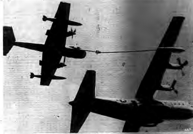
FILL 'ER UP!—An Army MOHAWK OV-1, left, is refueled in the air for the first time by a KC-130F HERCULES tanker during feasibility tests at the Naval Air Test Center, Patuxent River, Md. Modifications on the MOHAWK included two 300-gallon drop tanks; a refueling probe and nozzle mounted on the right side of the fuselage; a control panel and connection to the fuel system. Grumman Aircraft manufactures the MOHAWK for the Army. Photo, courtesy Lockheed.
