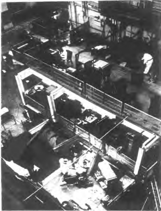
MAIN EXPERIMENTAL FACE of the Brookhaven National Laboratory Graphite Research Reactor, showing some of the experimental installations that utilize the neutrons produced by the chain reaction of fissioning uranium atoms in the reactor. At this face, there are 30 separate holes through the 5-foot thick heavy concrete shielding wall, available for experimental use.
